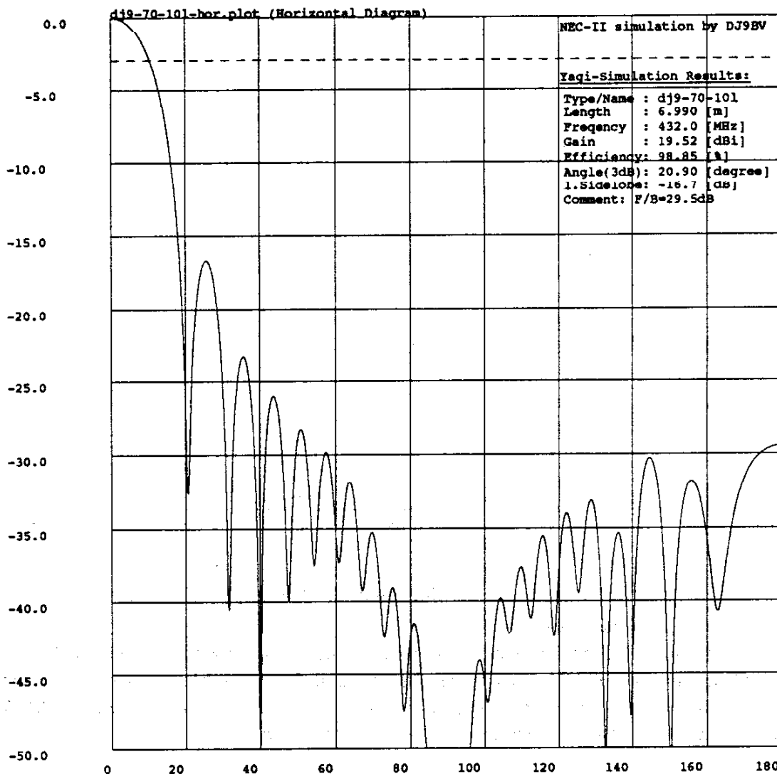
Bild/Figure 3: Horizontal Pattern of BV70-10L
