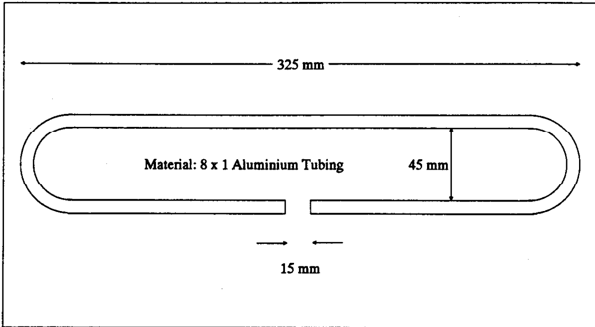
Bild/Figure 5: Dimensions of folded dipole for BV70
