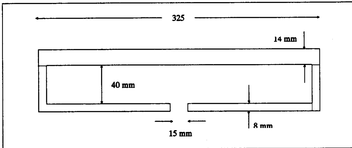
Bild/Figure 8: Transforming Folded Dipole for OPT70
