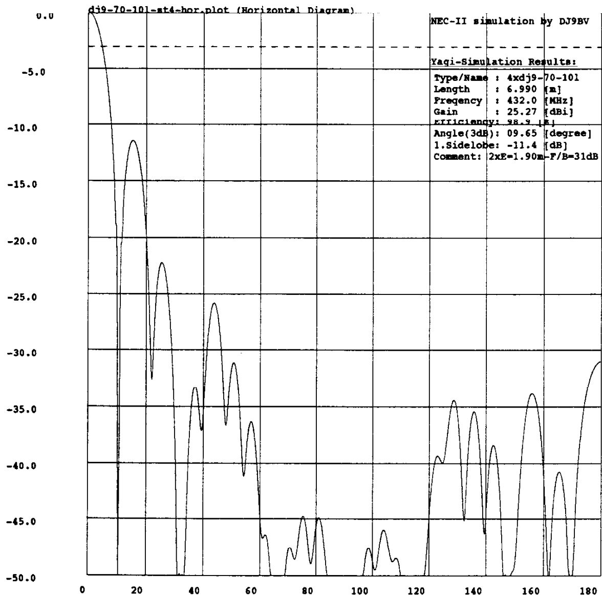
Bild/Figure 4: Horizontal Pattern of 4 x BV70-10L
