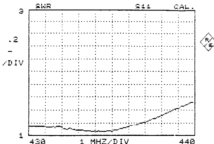
Bild/Figure 2: VSWR @ Frequency for BV70-8.5L
