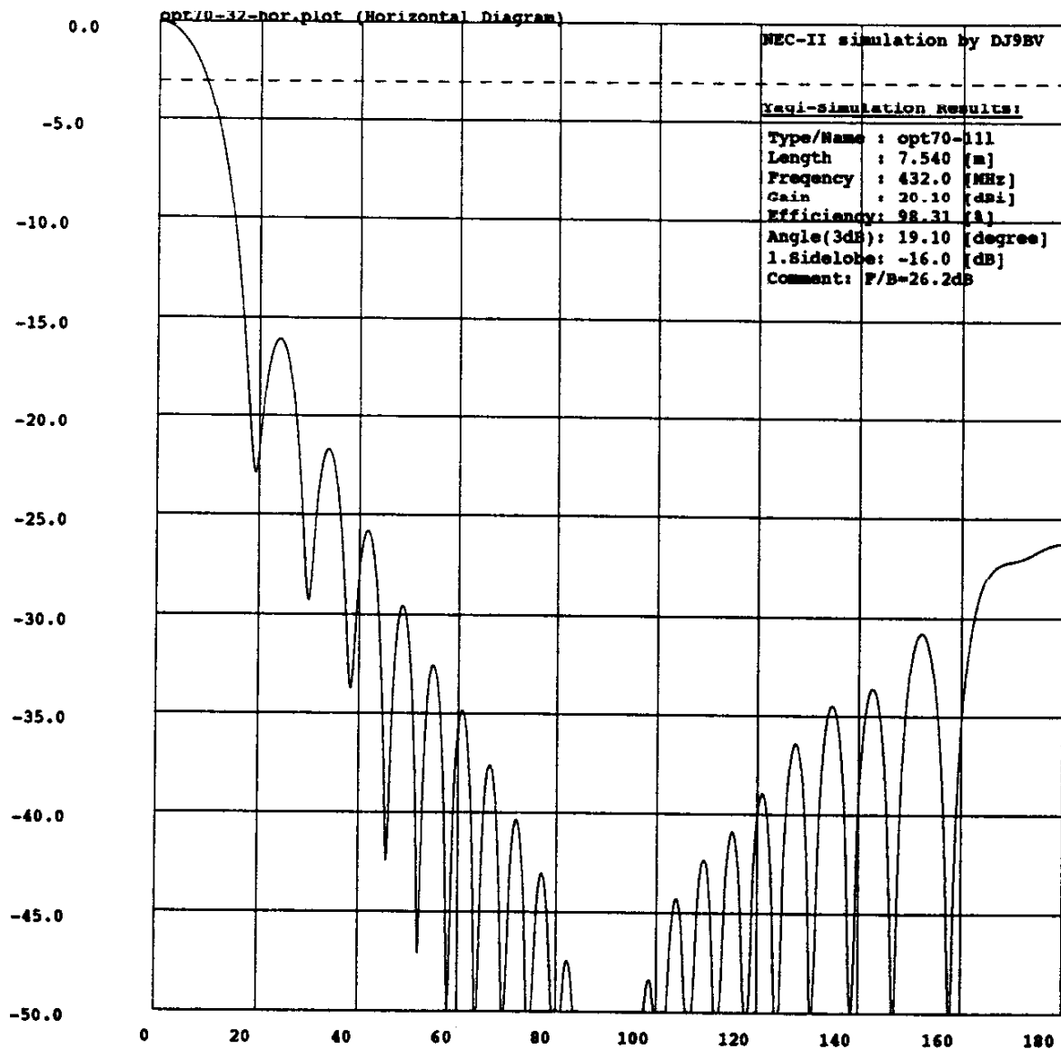
Bild/Figure 7: Horizontal Pattern of OPT70-11L
