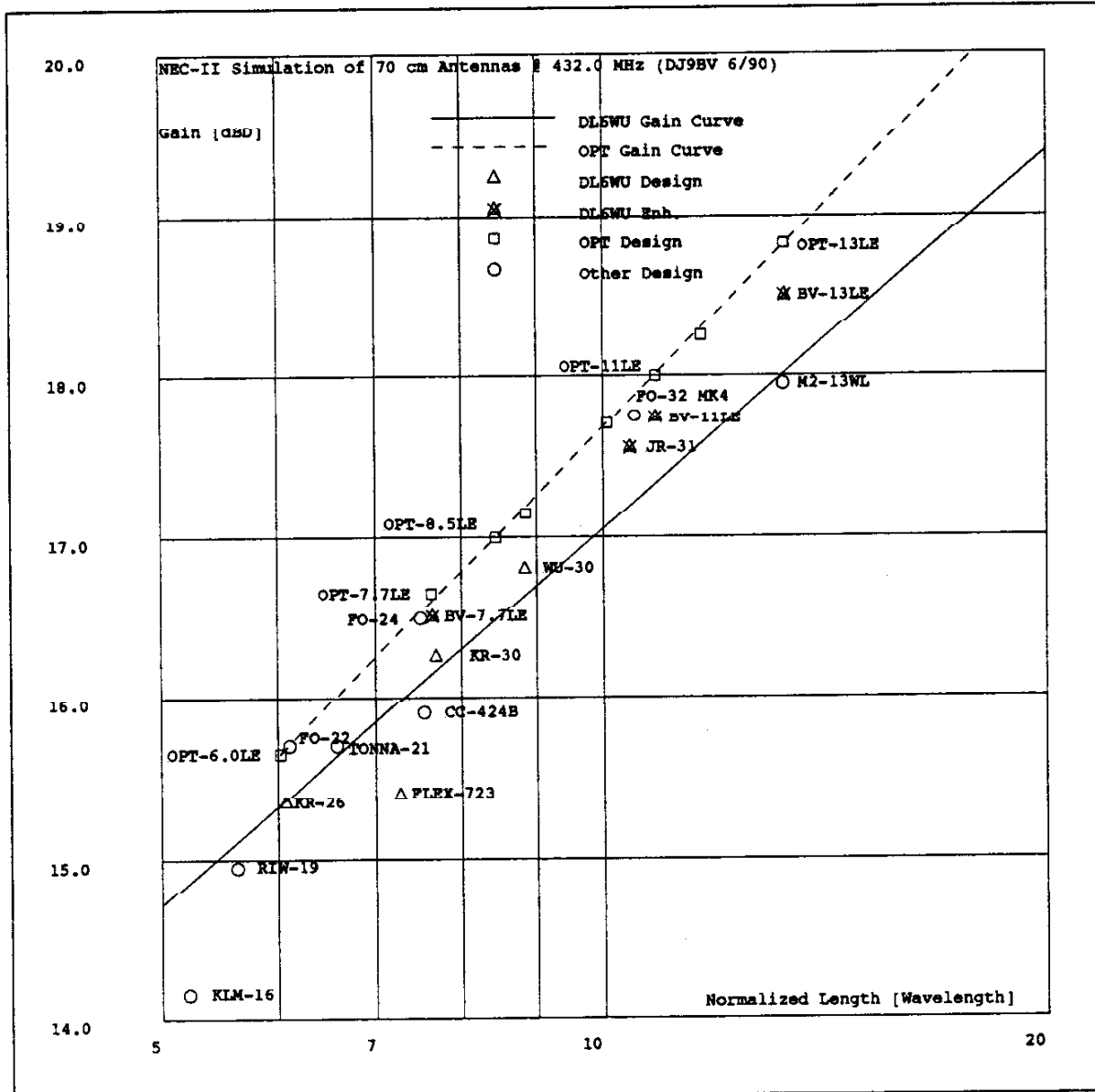
Bild/Figure 1: Gain versus Boomlength of 432 MHz Yagis
