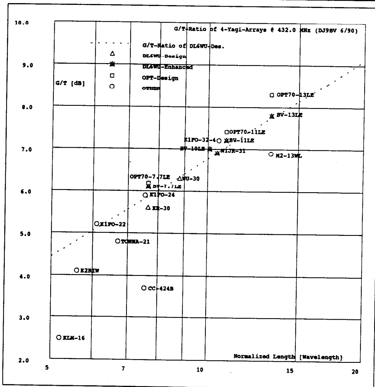
Bild/Figure 9: G/T-Ratio for 4-Yagi Arrays on 432
